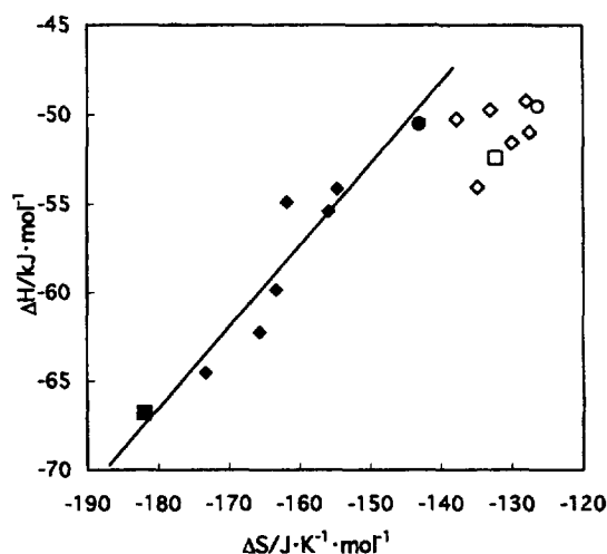
Figure 1. Enthalpy-entropy compensation plot for the complexation of ( S,R,R,S )-1 ( \diamond , \square and \circ ) and ( S,R,R,S )-2 ( \blacklozenge , \blacksquare and \bullet ) with amines.
