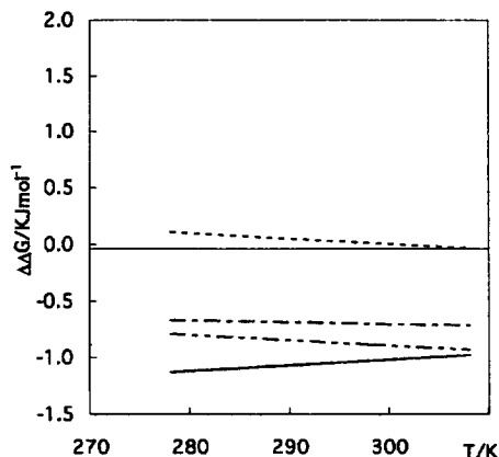
Figure 2. Temperature dependence of enantiomer selectivity for the complexation of ( S,R,R,S )-1 with amines; 16(···), 17(—), 18(···), 19(---).
